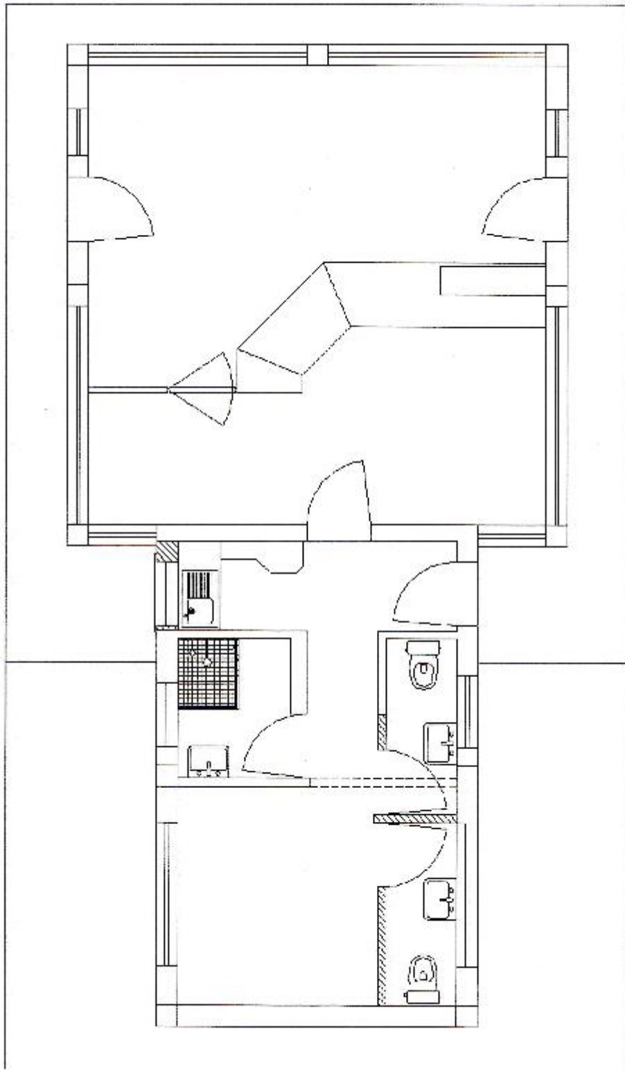
Figure 1 Gatehouse Layout
